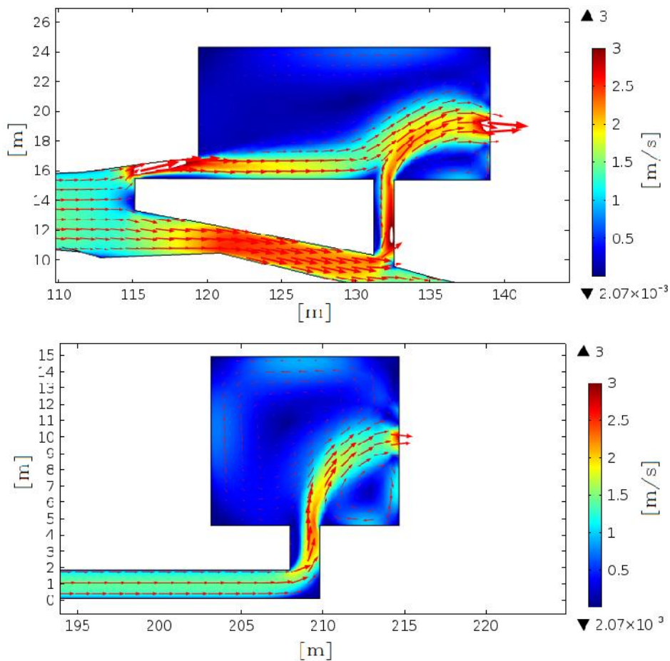
Figure 7. Detail of the results of Studio Aeolia for H = 95 m, DT = 10 for Villa Trento Carli (top), Villa Aeolia (bottom). Vector field and velocity magnitude are shown with a colour gradient according to the legend on the right m/s .
