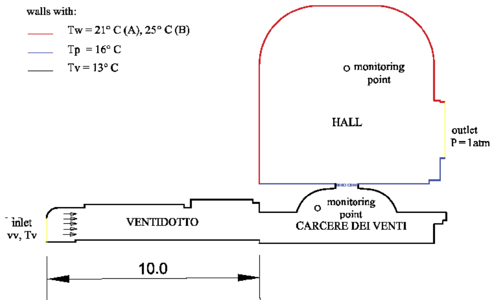
Figure 12. Geometry of the domain with the representation of the boundary conditions applied.
