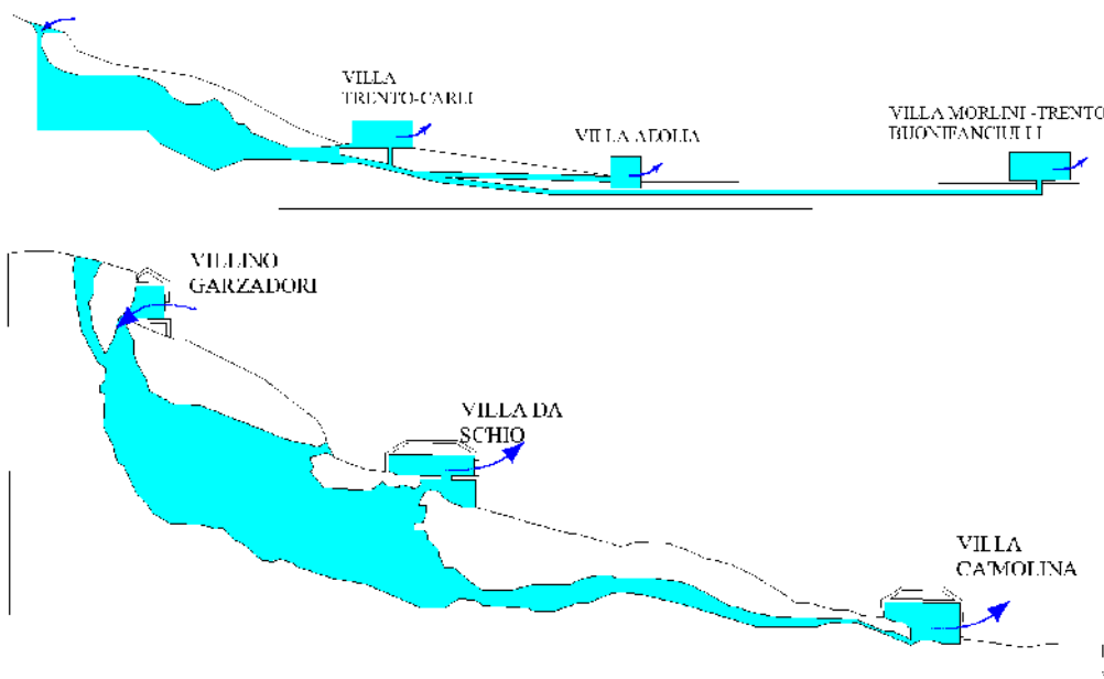
Figure 2. Schemes of the cooling systems: A group top B group bottom .
