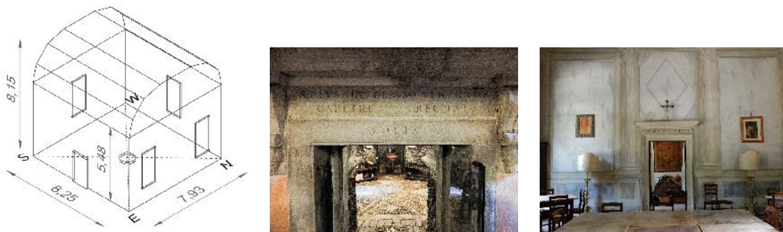
Figure 10. 3D geometry of Apollinea hall (left). The letters indicate the cardinal points. The room has four windows, the access door on the south-east wall, and a marble vent on the floor [50]. The inscription over the access door to the Carcere dei Venti: Aeolus hic clauso ventorum carcere regnat, Eolia center . The interior of Apollinea hall (right).
