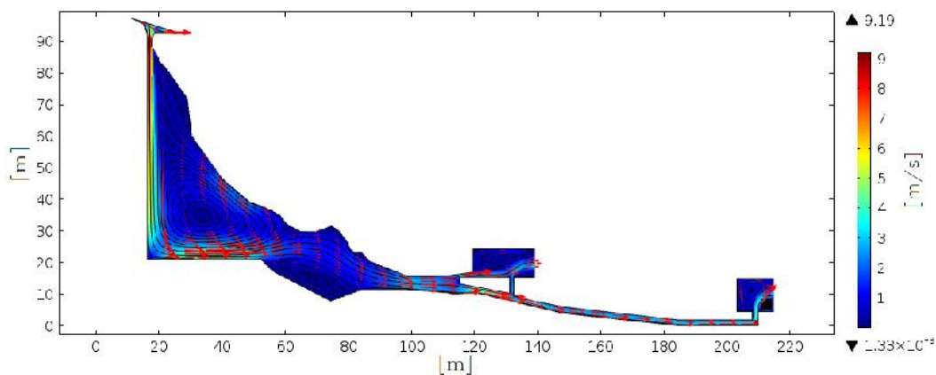
Figure 6. Results of Studio Aeolia for H = 95 \text{ m} , DT = 10 \text{ K} . Vector field and velocity magnitude are shown with a colour gradient according to the legend on the right \text{m/s} .
