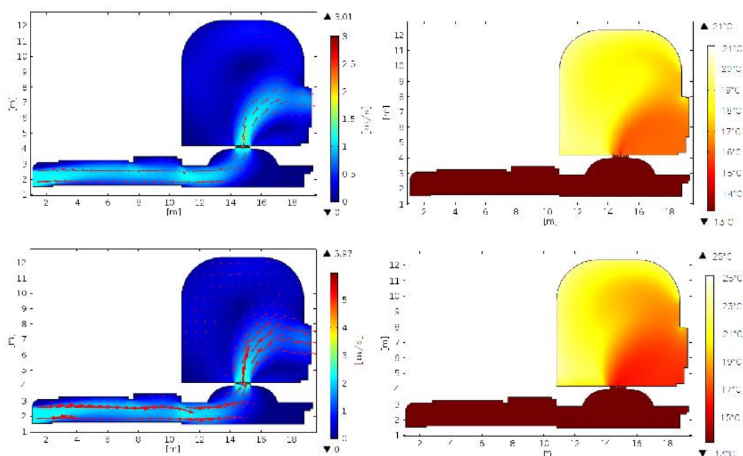
Figure 13. Case study A v_v 1.12 m/s): velocity field (m/s) (top left and temperature distribution top right). Case study B v_v 2.23 m/s): velocity field (m/s) (bottom left and temperature distribution bottom right).
