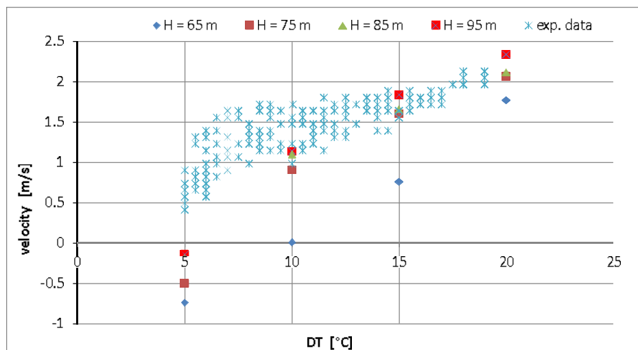
Figure 8. Results of Studio Aeolia for different altitudes H = 65\text{ m}, 75\text{ m}, 85\text{ m}, 95\text{ m} , in comparison with the experimental data of 46. The average air velocity was computed in the ventidotto at 10 m upstream of Villa Aeolia for variable outdoor indoor temperature difference DT .
