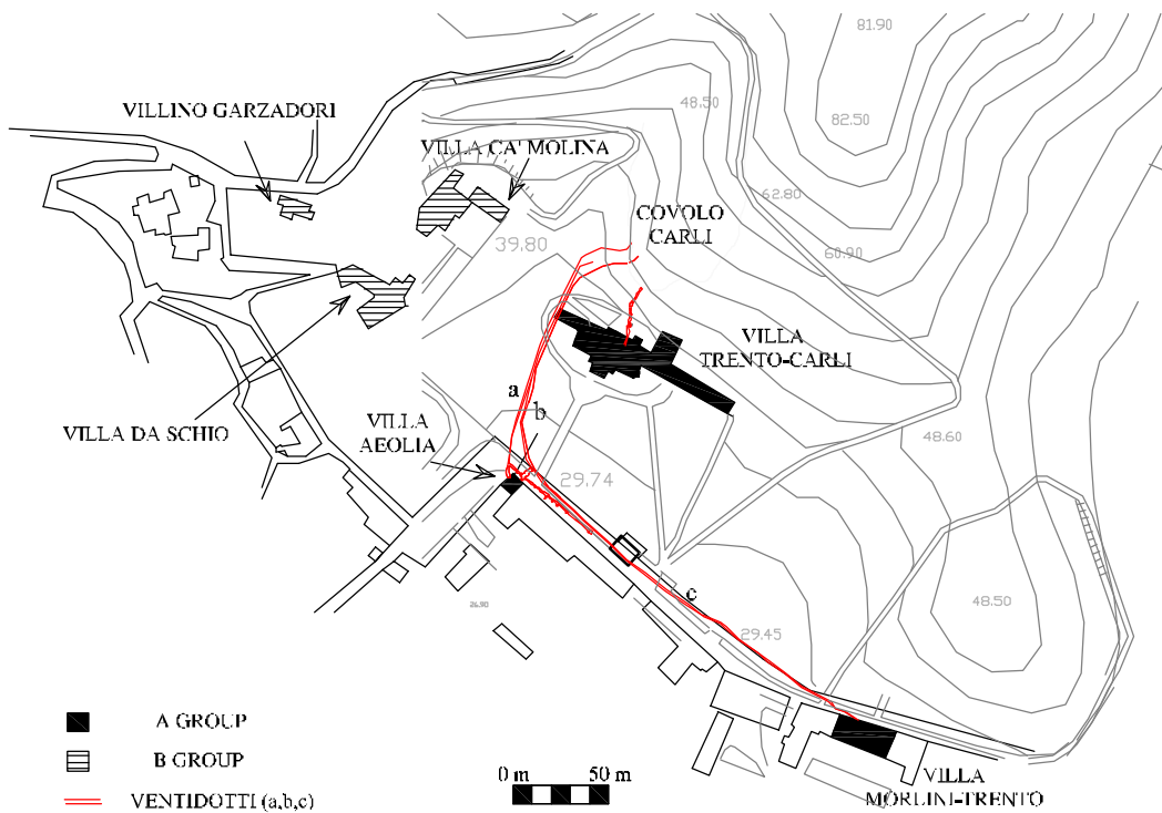
Figure 3. Plan of the area where the six villas are located (i.e., group A and group B). The artificial underground ducts i.e., ventidotti are in red.
