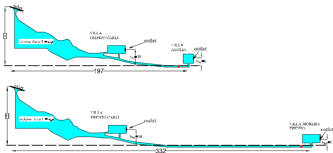
Figure 5. Geometry of the model of Studio Aeolia top with Villa Trento Carli and Villa Aeolia and the model of Studio Morlini Trento below with Villa Trento Carli and Villa Morlini Trento with boundary conditions. We indicate the position of the inlet and outlet, the height of the openings of the villas, and the presence of the volume force. On the solid boundaries we applied the wall functions. The units are in meters. The red dot indicates the monitor points of the computation to reach the steady solution, and its abscissa corresponds to the position where we computed the mean air velocity of the air flow in the ventidotto.
