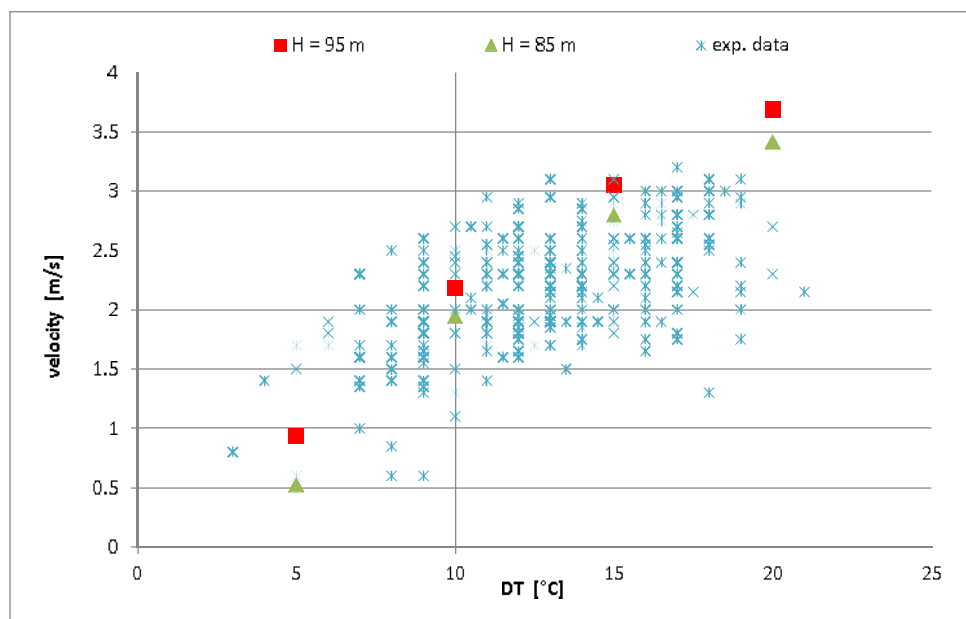
Figure 9. Results of Studio Aeolia for different altitudes H = 85\text{ m}, 95\text{ m} , in comparison with the experimental data of 48. The average air velocity was computed in the ventidotto at 30 m upstream to Villa Aeolia for variable outdoor indoor temperature difference DT .
