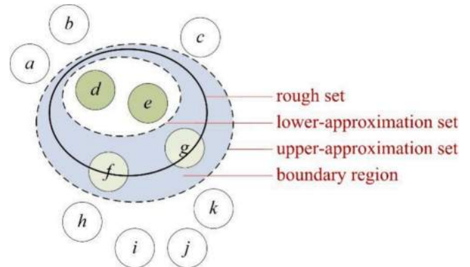
Fig. 6. Representation of a rough set.
