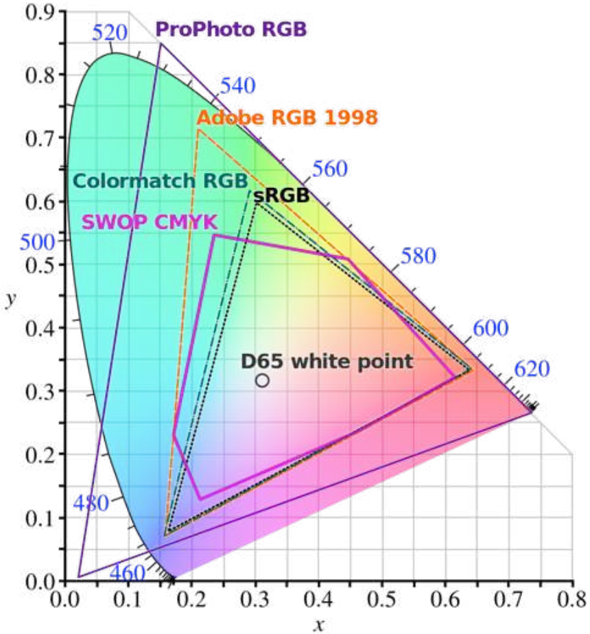
FIG. 53: Comparison of some RGB and CMYK chromaticity gamuts on a CIE 1931 XY chromaticity diagram < https://en.wikipedia.org/wiki/Color_space#/media/File:CIE1931xy_gamut_comparison.svg > (accessed 31.10.2024).
