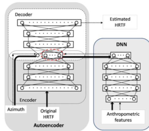
Figure 1: Architecture proposed by Chen et al., with HRTF autoencoding and latent representation estimation from anthropometry with a DNN. Solid arrows indicate the training process, dotted arrows indicate usage, and the red dashed oval highlights the latent space. Figure reproduced from [5].
