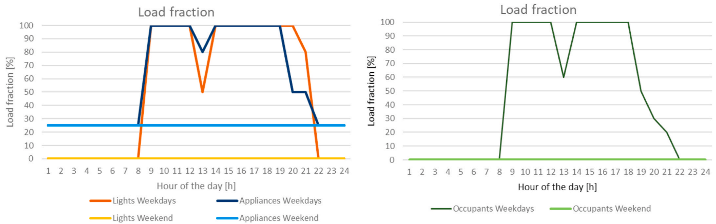
Fig. 12. Load fraction for occupants, lighting, and electric appliances according to EN 18523-1 [102] for office use.
