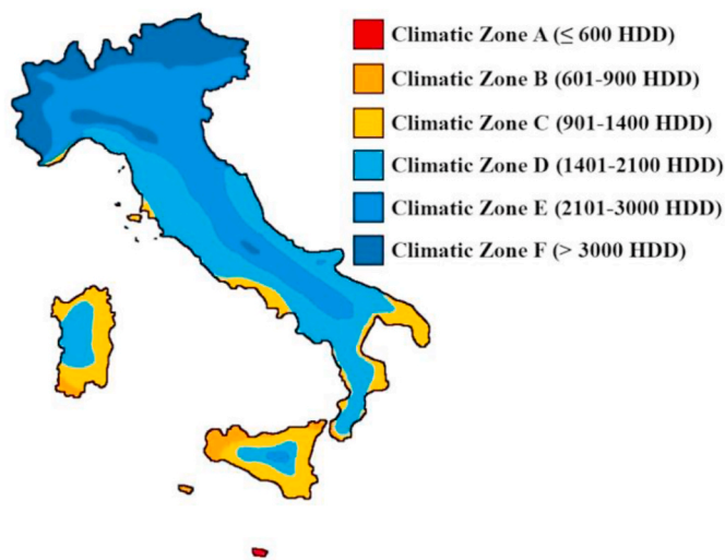
Fig. 4. Italian climatic zone distribution [59].
