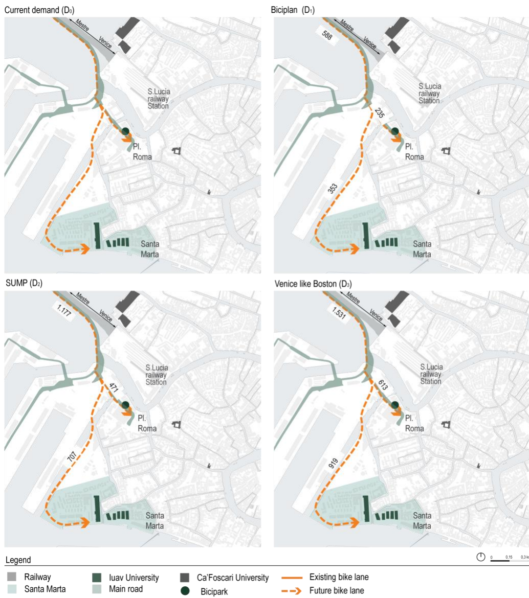
Figure 3. Current and future daily bike flows along Liberty bridge to Santa Marta and Piazzale Roma in different scenarios (D k )
