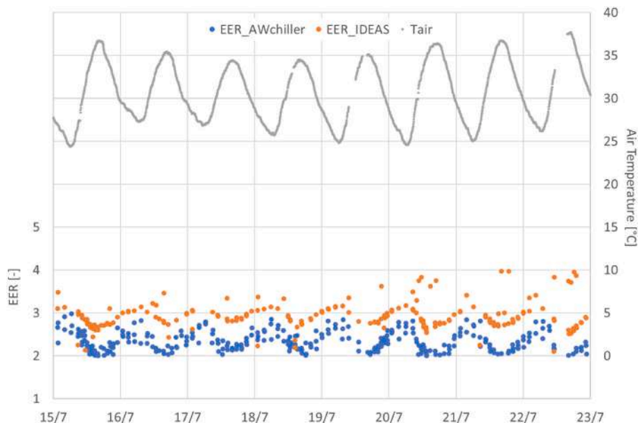
Fig. 11. Comparison between EER values of AW chiller and IDEAS system - From 15/07/22 to 23/07/22.
