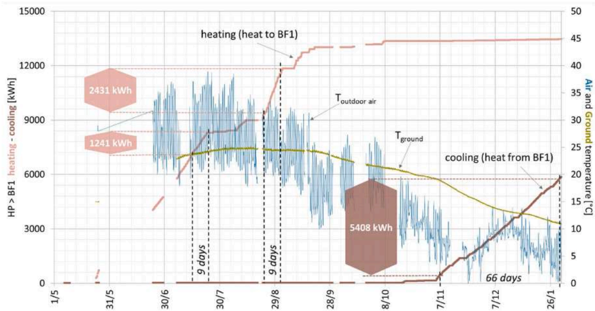
Fig. 9. Heat load – Primary loop Source side.
