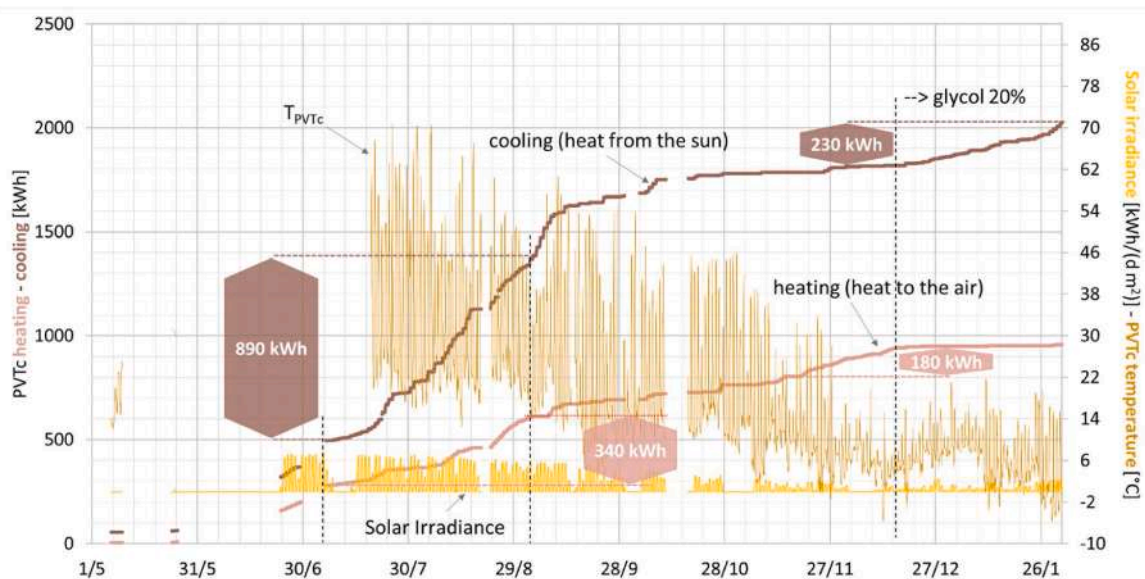
Fig. 7. Heat fluxes at the PVTc loop.
