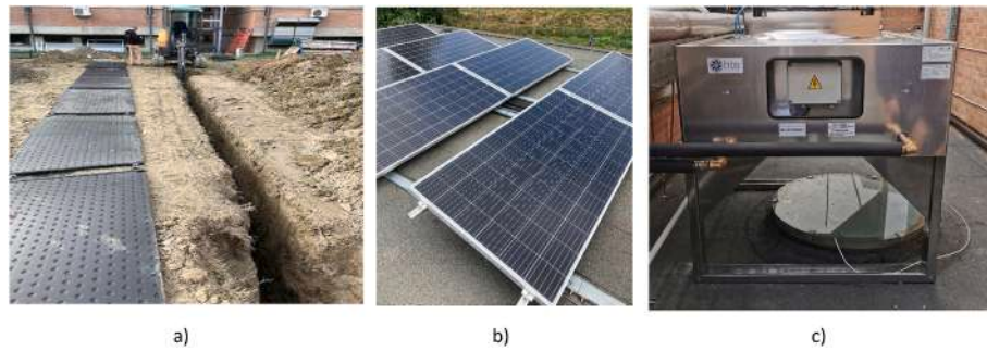
Fig. 2. Pictures of the IDEAS systems: a) GHXs installation b) PVT c field c) AHX (drycooler).
