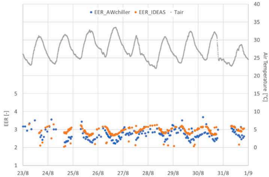
Fig. 12. Comparison between EER values of AW chiller and IDEAS system - From 23/08/22 to 01/09/22.
