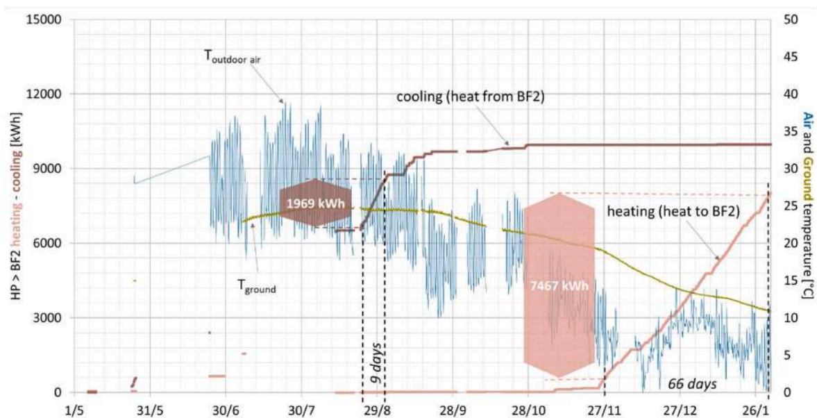
Fig. 10. Heat load – Primary loop User side.
