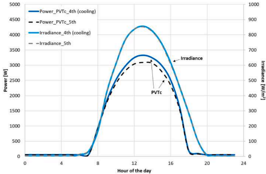
Fig. 8. Electricity production with and without cooling at the PVT c loop.
