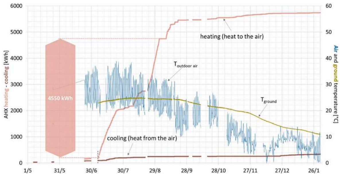
Fig. 6. Heat fluxes at the AHX loop.
