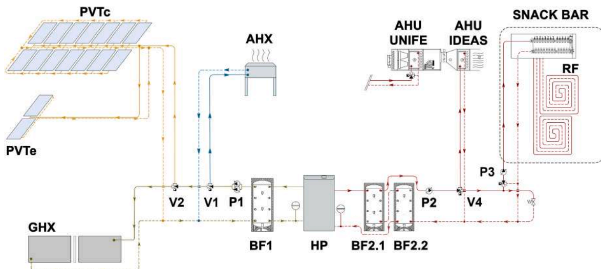
Fig. 3. Piping and instrumentation diagram of the IDEAS experimental plant.
