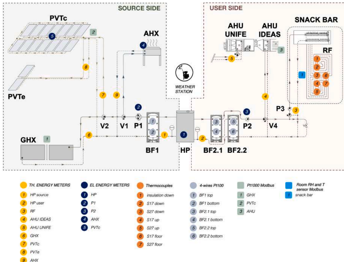
Fig. 4. Measuring devices installed in the IDEAS experimental plant.
