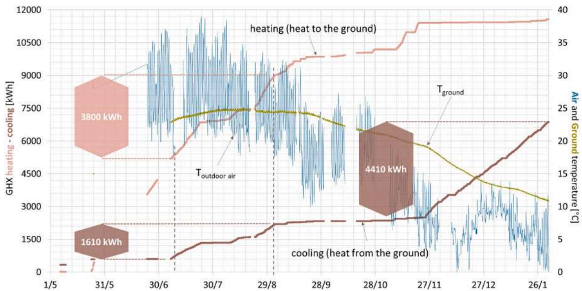
Fig. 5. Heat exchanged with ground, external air temperature and ground temperature.
