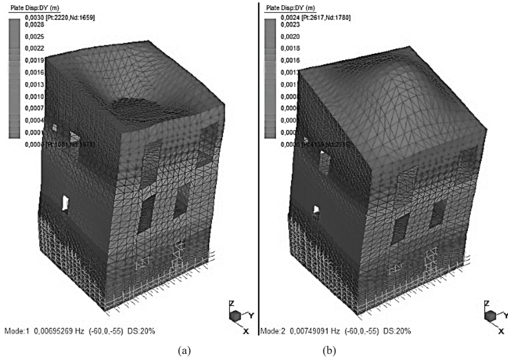
Fig. 8 Modal analysis: (a) Mode 1, (b) Mode 2
