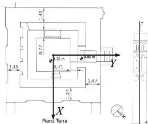
Fig. 11 Modal analysis axes reference
