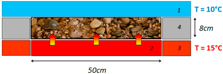
Fig.1. The guarded hot plate device tested for measuring thermal properties of gravels. 1: cold plate; 2: hot plate; 3: protection material to the hot plate; 4: protection ring of insulation material (guard), used to impose a one-dimensional heat flux through the sample.
