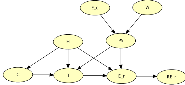
Figure 1: Bayesian network for reported evidence applicable for transfer from PoI to the victim or from victim to PoI. Node descriptors are given in Table 1 with definitions that depend on a direction of transfer from the PoI to the victim.
