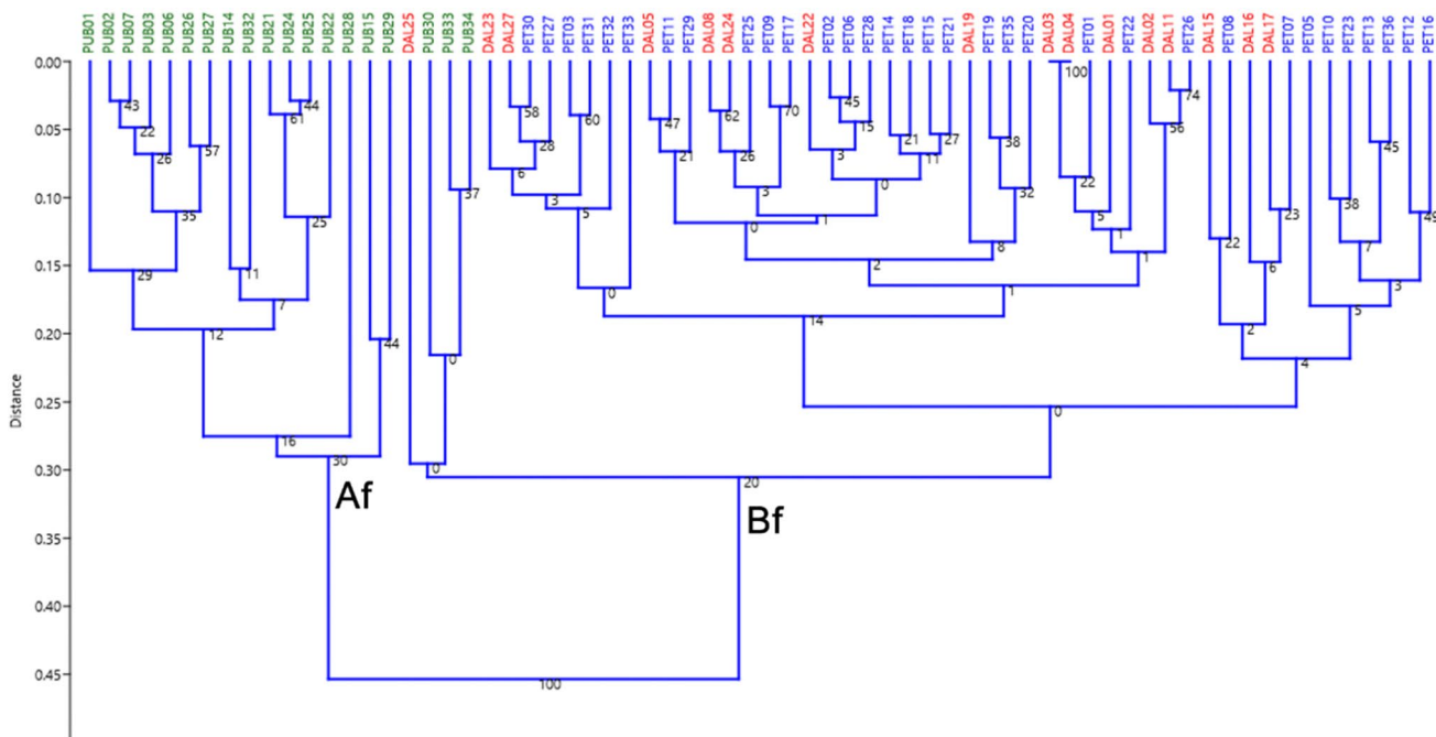
Fig. 4 Clustering of the 68 trees using the eleven variables of fruits. Gower distance and UPGMA; 100 bootstraps. Cophenetic correlation=0.872. Q. petraea (blue), Q. pubescens (green), and Q. dalechampii (red)
