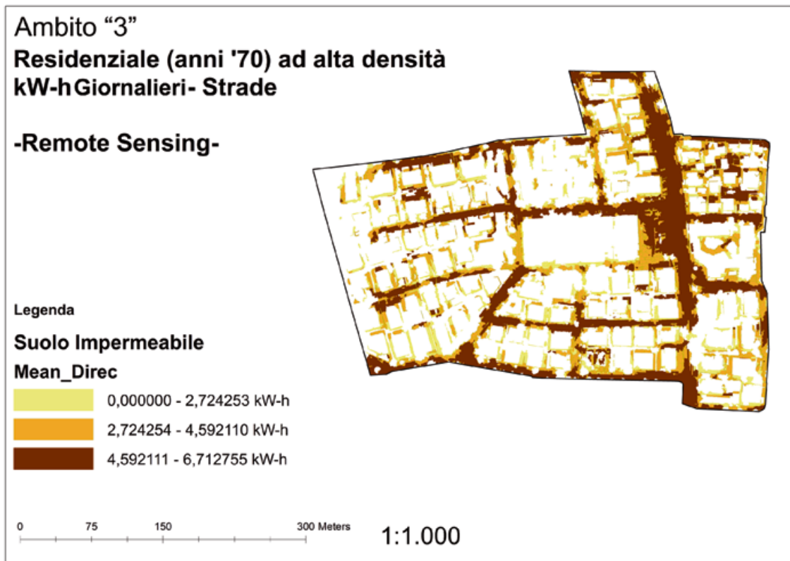
Fig. 8.9 High density residential neighbourhood (1970's) Daily kW/h/roads
